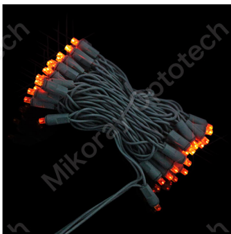
5mm LED Orange/Green Cord Model:MH2-50-5MM-O Cord: 22 AWG Voltage: 120V
