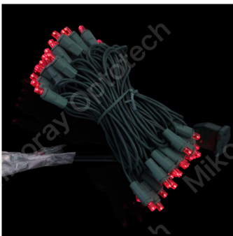
5mm LED Red/Green Cord Model:MH2-70-5MM-R Cord: 22 AWG Voltage: 120V
