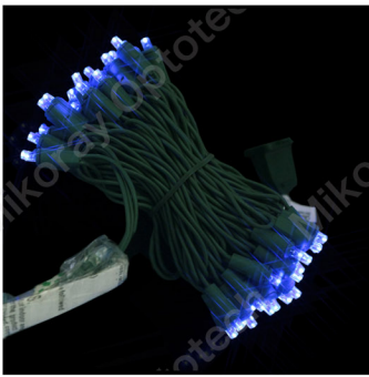
5mm LED Blue/Green Cord Model:MH2-70-5MM-B Cord: 22 AWG Voltage: 120V
