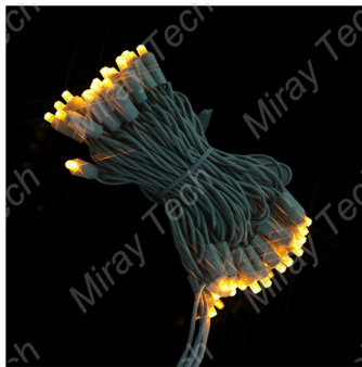
5mm LED Yellow/Green Cord Model:MH2-70-5MM-Y Cord: 22 AWG Voltage: 120V
