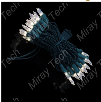
Mini LED Warm White/Green Cord Model:MH2-70-Mini-WW Cord: 22 AWG Voltage: 120V
